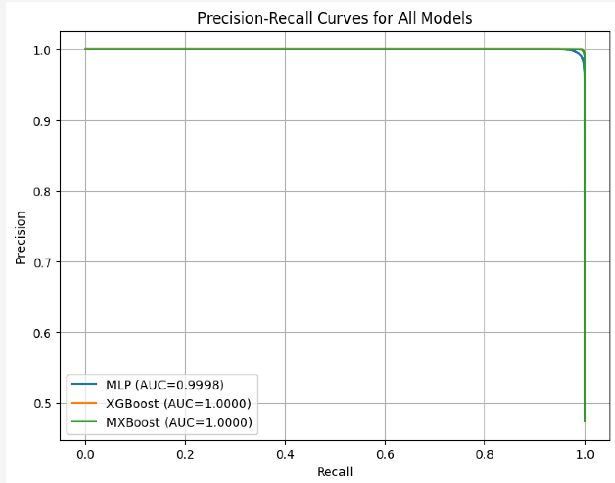
Fig 11: Precision-Recall Curve
